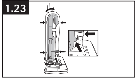
While wrapping hose in a clockwise direction, push it firmly into rack at areas shown. Note: To keep hose secured, place round end of hose below bottom extension.
